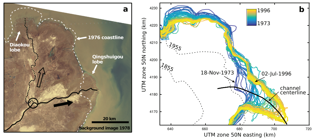
Figure 4. (a) Landsat 2 satellite composite image (1978) with superimposed coastline trace from a 1976 Landsat 2 image (white dashed line). In 1976, an engineered avulsion at the small open circle changed the channel course from the north (dotted line, open arrow) to the east (solid line, solid arrow). When compared to the 1976 coastline, the underlying satellite image shows retreat of the former delta lobe in the north (Diaokou lobe) and development of a new lobe to the east (Qingshuigou lobe); development of the Qingshuigou lobe continued without subsequent avulsion until 1996. (b) Coastline traces derived from historical record and satellite images. Traces from 1973 to 1982 are from manually georeferenced Landsat 1–3 sensor measurements. Traces from Landsat 4, 5, 7, and 8 are derived by automatic image processing (details and positional error information are included in text). Thick black line represents a portion of the channel centerline during the progradation of the Qingshuigou lobe.
