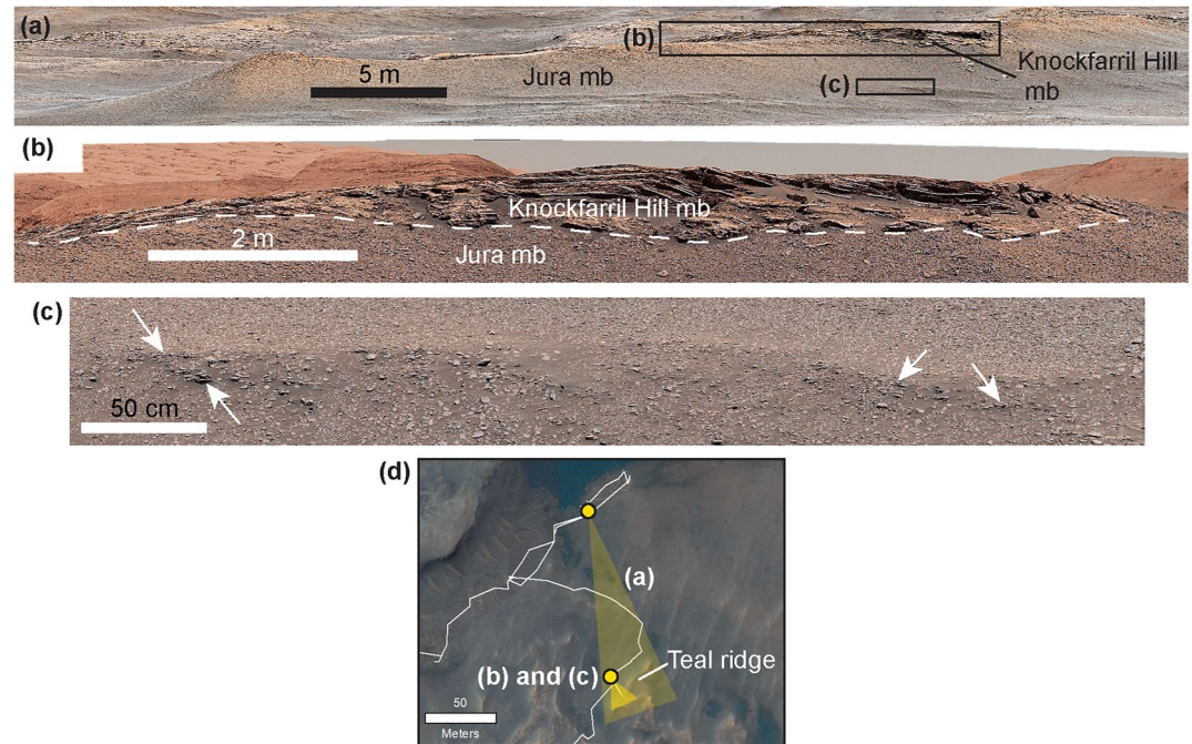
Figure 14. Views of Teal ridge observed with Mastcam. View is to the east. (a) Teal Ridge in a Mastcam right-eye mosaic acquired on sol 2365. Black boxes show the location of areas shown in panels (b) and (c). (b) Contact (white dashed line) between cross-bedded Knockfarril Hill member sandstone (cross-strata are traced in white) and underlying GT Jura member at the cap of Teal ridge in a Mastcam left-eye mosaic acquired on sol 2437. (c) Rubbly clasts, possibly eroding from in-place exposure, along the flank of Teal ridge in a Mastcam right-eye mosaic acquired on sol 2437. White arrows point to small in-place portions of the outcrop. Image credit: NASA/Caltech-JPL/MSSS. (d) Approximate viewsheds for the Mastcam mosaics displayed in panels (a–c). The center coordinate (lat, lon) of the area shown in High Resolution Imaging Science Experiment is -4.7274, 137.3837 .
